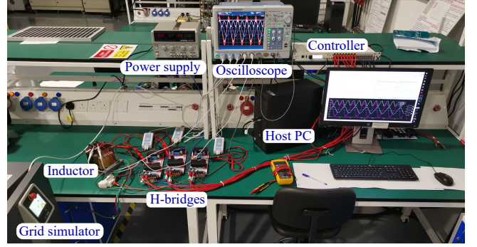
Fig. 4. Experimental setup.
